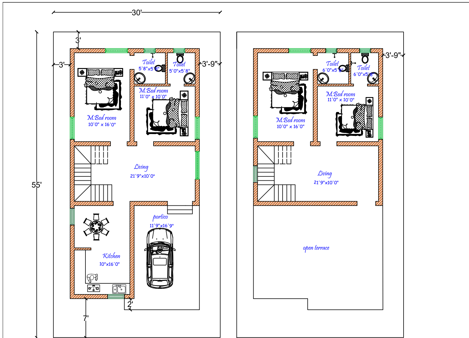
FIRST FLOOR PLAN 657 s.ft
